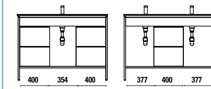
CENTERED SINK WASHBASIN (1 or 2 modules) / DOUBLE SINK WASHBASIN
