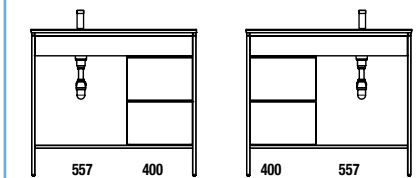
WASHBASIN MODULE ON THE RIGHT / WASHBASIN MODULE ON THE LEFT
